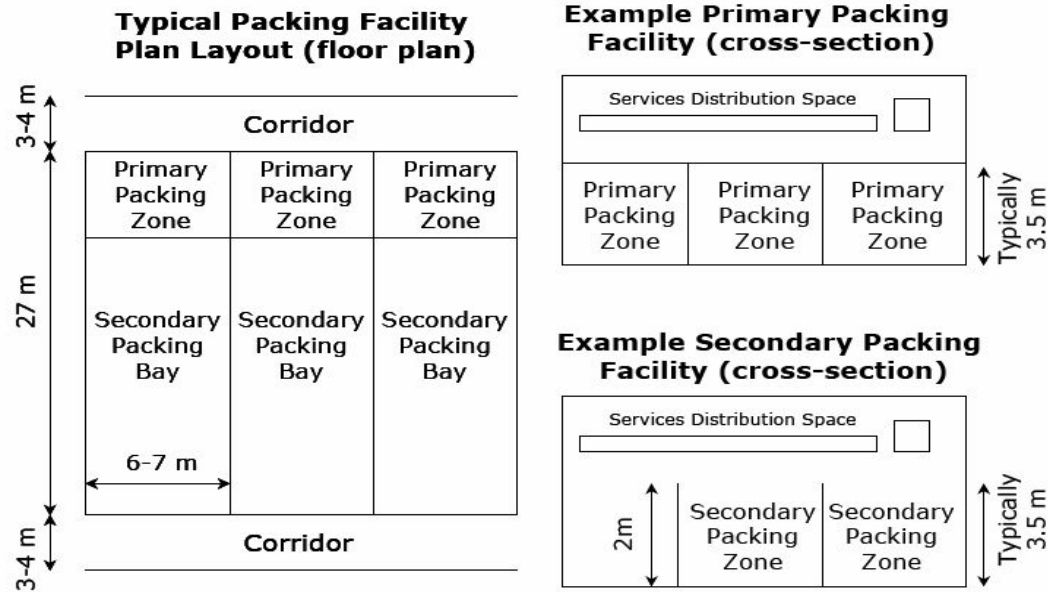
Diagram 1: Example Packing Facility Design
